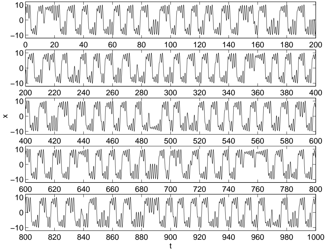
Figure 6: A simulation of Chua's circuit: x versus time t in seconds.
