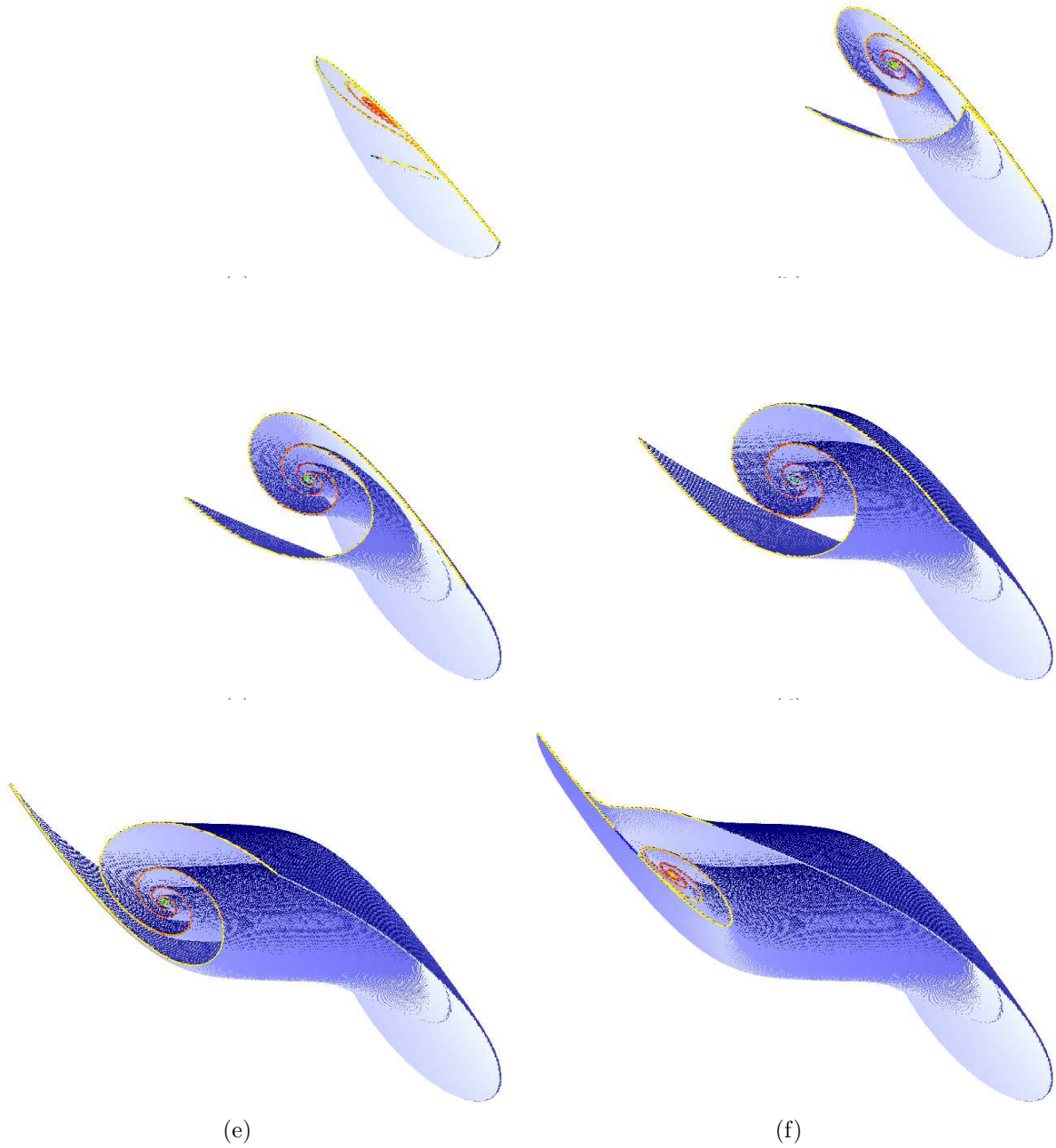
Figure 3: Cutting planes illustrating the structure of the attracting set in Chua's circuit as well as the natural invariant measure (27 subdivisions, 877346 boxes). In the cutting planes the density ranges from green (low density) \rightarrow red \rightarrow orange \rightarrow yellow (high density).
