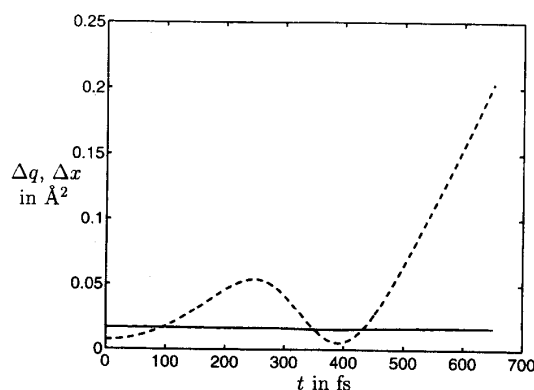
FIG. 6. Evolution of variances \Delta q (dashed) and \Delta x (solid) of the full QD wave packet. Note the disintegration of the wave packet in q direction in which no attractive potential is present. It is increasing as long as the particle is moving "free" and decreasing during the collision.
