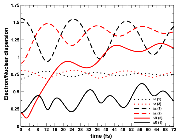
FIG. 6: (Color online) Electronic and nuclear dispersions as functions of time: the nuclear one \Delta R(t) (solid), the electronic one in z -direction \Delta z(t) (dashed) and r -direction \Delta r(t) (dotted). The dynamics for the outer initial condition (1) are in black, while those for the inner one (2) are in red/gray colors.
