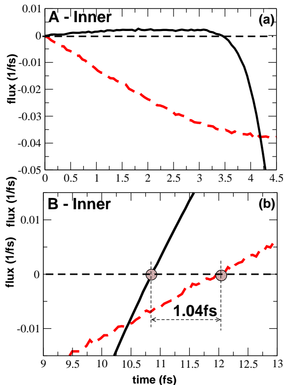
FIG. 8: (Color online) ZOOMS of regions A and B of Figure 4(b) for the nuclear flux (solid) and the electronic one (dashed). Until 3.5fs, the electron and nuclei move in opposite directions (A-Inner). At later time (B-Inner), the nuclei return and the electron follows with a delay of 1.04fs.
