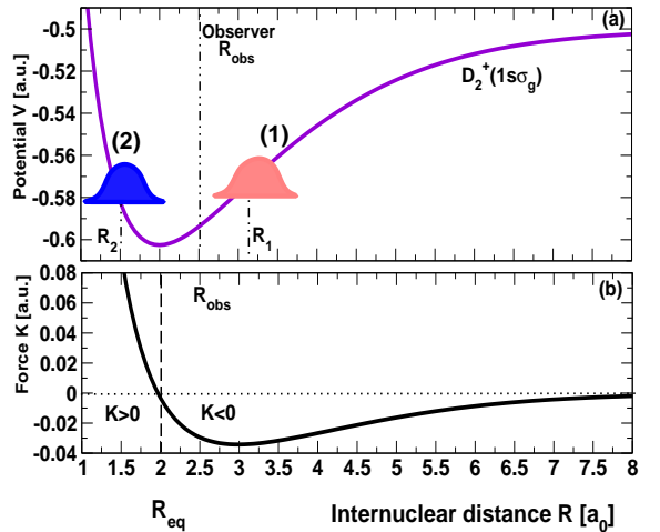
FIG. 1: (Color online) The upper panel (a) shows the potential energy surface V(R) of D_2^+ . The outer (1) and the inner (2) regions denote the initial locations of the nuclear wavepackets centered at R_1 and R_2 , respectively. These wavepackets have been promoted to D_2^+ from the ground state of D_2 . The dot-dashed vertical lines indicate the location of our observer R_{obs} . The lower panel (b) shows the force K = -dV/dR acting on the nuclear wavepacket. The equilibrium internuclear distance R_{eq} is indicated by a dashed vertical line.
