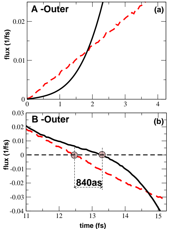
FIG. 7: (Color online) Zooms of regions A and B of Figure 3(b) for the nuclear flux (solid) and the electronic one (dashed). The electron and nuclei start moving synchronously (A-Outer). At later time (B-Outer), the electron returns first and after 840as, the nuclei follow.
