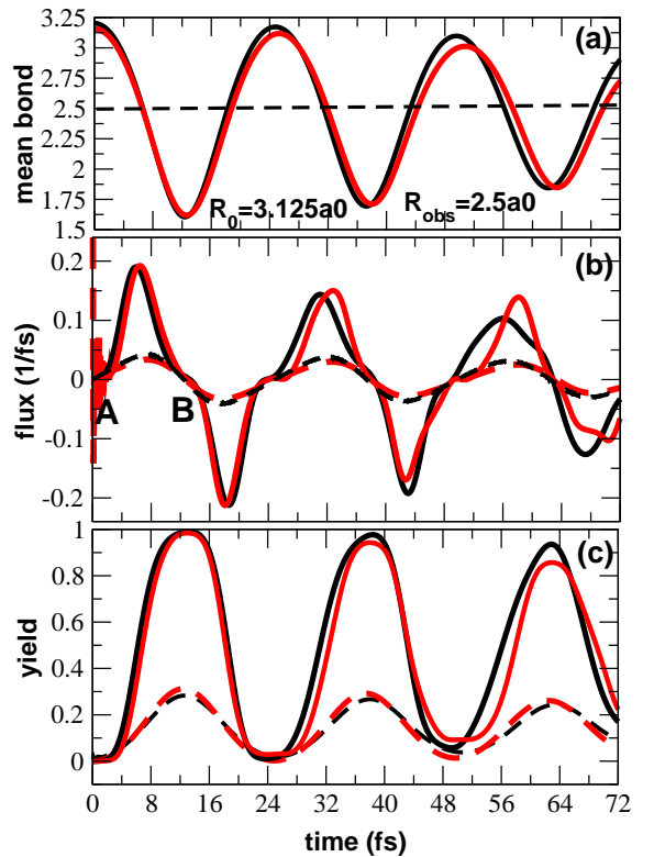
FIG. 3: (Color online) Dynamics for the outer initial condition centered in R_1 = 3.125a_0 . The underlying simulations solve the full molecular Schrödinger equation (red/gray) or use the BO approximation (black). Nuclear quantities are plotted by solid lines, electronic ones by dashed lines. The upper panel (a) shows the mean bond length. Additionally, the observer location at R_{obs} = 2.5a_0 is indicated as a dashed horizontal line. The lower two panels show the evolution of the electronic and nuclear fluxes (b) and the yields (c). The dynamics within the regions marked by A and B are more thoroughly discussed in Sec. IV B.
