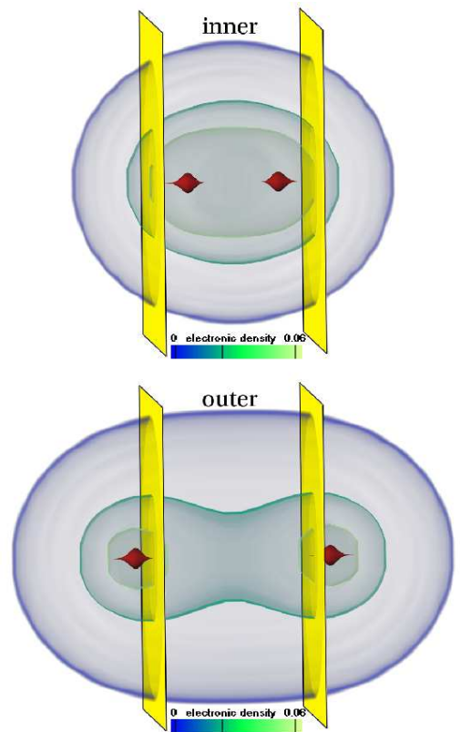
FIG. 2: (Color online) Visualization of the initial states as defined in Fig.1. The upper panel represents the inner initial state and the lower panel the outer one. The electronic densities, with its associated color code, surrounds the nuclear density in red/gray color. The space inside the two parallel planes of the observer A_{obs} , in yellow/light-gray color, corresponds to the volume of the observer V_{obs} . The two planes are located at z_{obs} = \pm R_{obs}/2 , where R_{obs} is the distance separating the two planes. This visualization has been created using the academic system ZIBAmira, a superset of its commercial version Amira[14].
