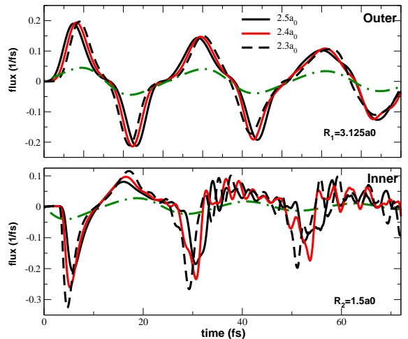
FIG. 5: (Color online) Robustness of the electronic and nuclear flux with respect to the observer position. The nuclear flux evolution for the outer and the inner initial state are shown in the upper and the lower panel, respectively. The three different locations of the observer are R_{obs} = 2.3a_0, 2.4a_0 , and 2.5a_0 . Both panels also plot the electronic flux (dot-dashed), which is insensitive to the considered variations of the observer plane.
