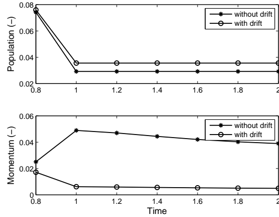
(c) The accuracy of the single switch algorithm for the population and momentum expectation value of the lower level.
