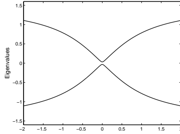
(a) The eigenvalue surfaces of (3.1).
