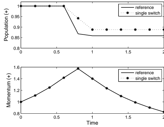
(b) The dynamics of the population and the momentum expectation value for the upper level.
